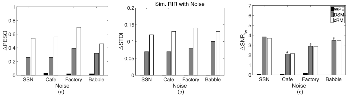
Fig. 6. (a) \Delta PESQ, (b) \Delta STOI, (c) \Delta SNR fw results using simulated RIRs and background noise. The improvement relative to the unprocessed noisy-reverberant speech is shown. '#' indicates that the differences from cRM results are not statistically significant according to a one-way ANOVA test with 5% confidence interval.
