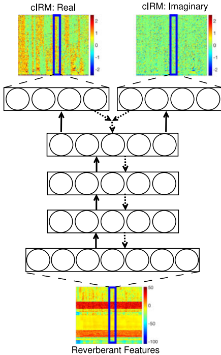
Fig. 3. (Color Online). Network structure of the DNN that estimates the complex ideal ratio mask.
