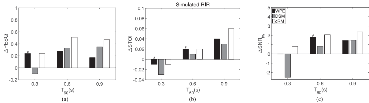
Fig. 4. (a) \Delta PESQ, (b) \Delta STOI, (c) \Delta SNR fw results using simulated RIRs. The improvement relative to the unprocessed reverberant speech is shown. '#' indicates that the differences from cIRM results are not statistically significant according to a one-way ANOVA test with 5% confidence interval.
