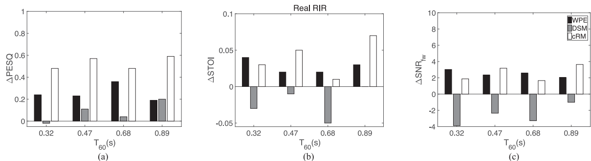
Fig. 5. (a) \Delta PESQ, (b) \Delta STOI, (c) \Delta SNR fw results using real RIRs. The improvement relative to the unprocessed reverberant speech is shown. All differences from cIRM results are statistically significant according to a one-way ANOVA test with 5% confidence interval.
