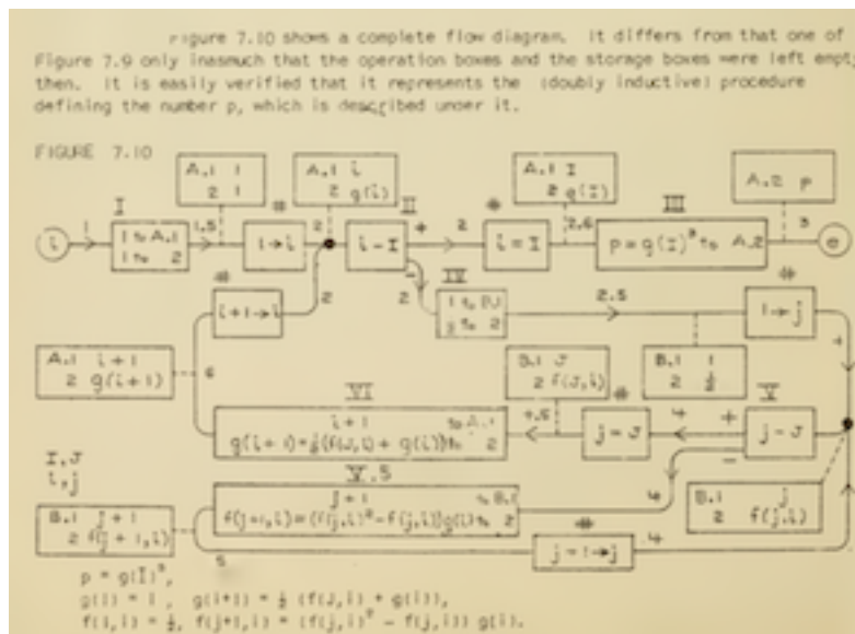
Figure 2: An original flow diagram from Goldstine and von Neumann’s 1947 “Planning and Coding of Problems for an Electronic Computing Instrument.”
