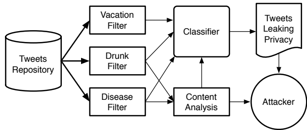
Figure 1: Architecture of our privacy detection approach. The three filter modules identify topical tweets based on keyword matching. These tweets are then fed through classifiers to detect sensitive tweets. The content analysis module characterizes the nature of privacy leaks for each of the three categories (vacation, drunk, and disease tweets).
