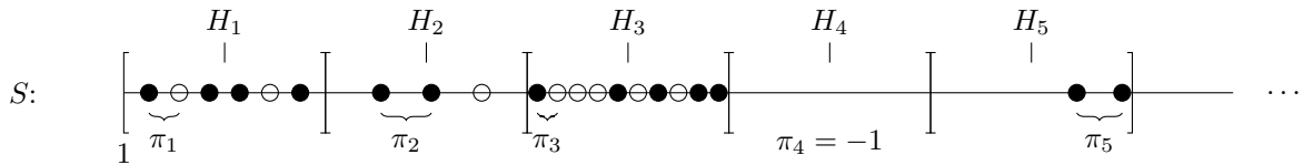
Figure 1 Observe that all dots in each interval are equally spaced after the first. These dots represent \mathcal{T}^c : the black dots represent \mathcal{T} , while the white dots are added to convert the irregularly spaced black dots into regularly spaced dot sequences.
