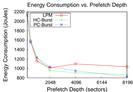
Figure 6: Disk energy consumption vs. prefetch aggressiveness (700MB memory)
